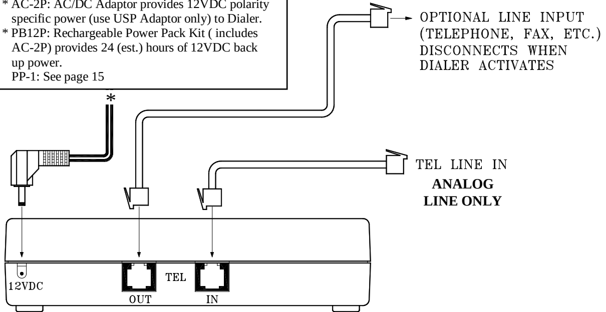
POWER & TELEPHONE LINE INTERFACE
