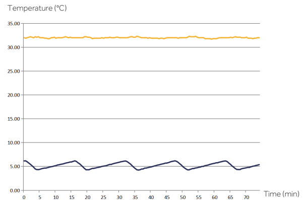
Stability Curve
