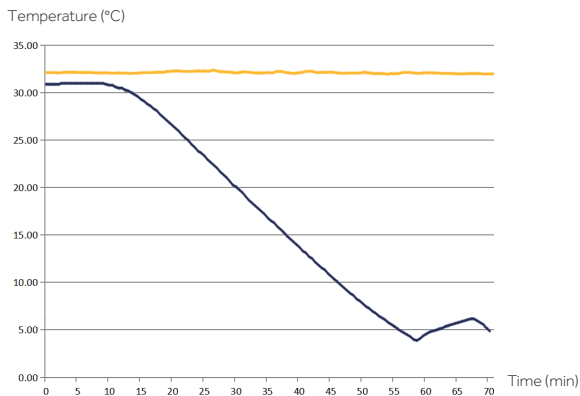
Cooling Down Curve
