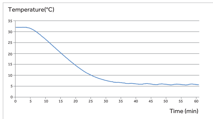
Refrigerator Stability Curve
